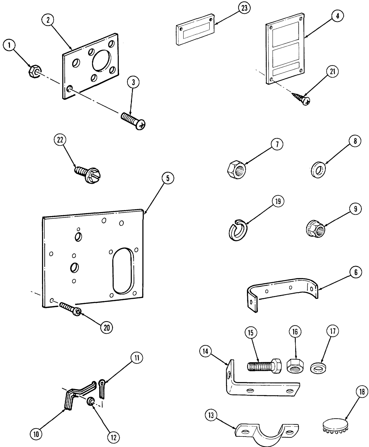
Figure 3. Modification Kit 12301498.
