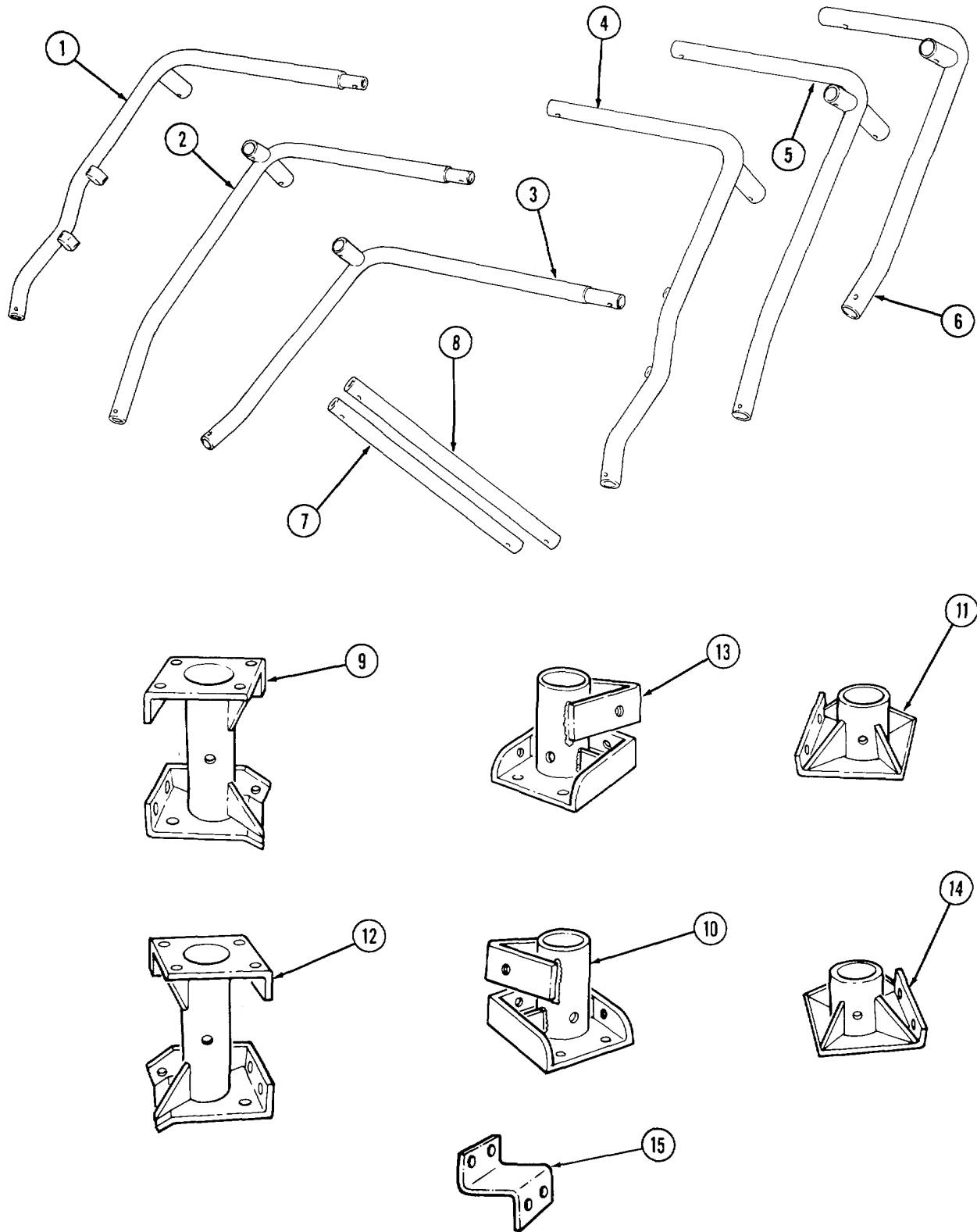
Figure 1. Modification Kit 12301498.
