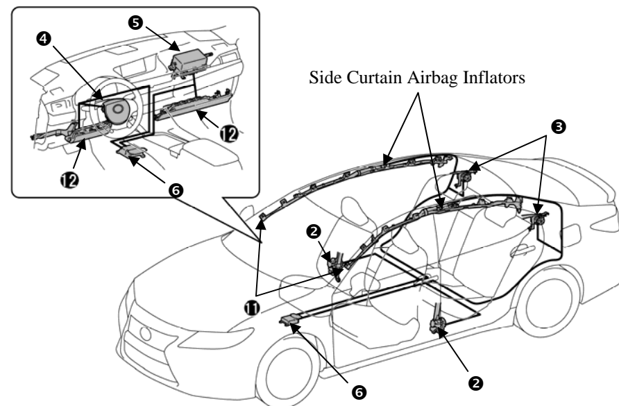
Standard Frontal Airbags, Seat Belt Pretensioners, Knee Airbags, Side Curtain Airbags
